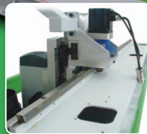
Ground helical rack and pinion and THK guides for Y axis
